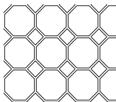
8" Diamond Tile Tile Size 195 x 195 Diamond 75 x 75
